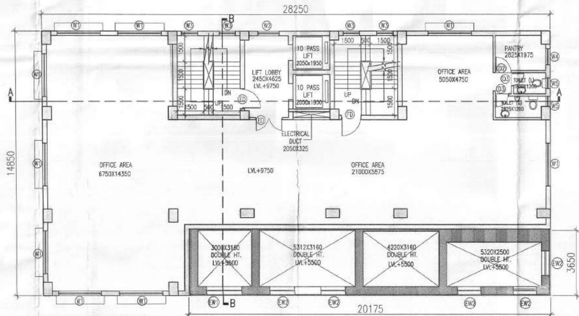
THIRD FLOOR PLAN SCALE - 1 : 100
